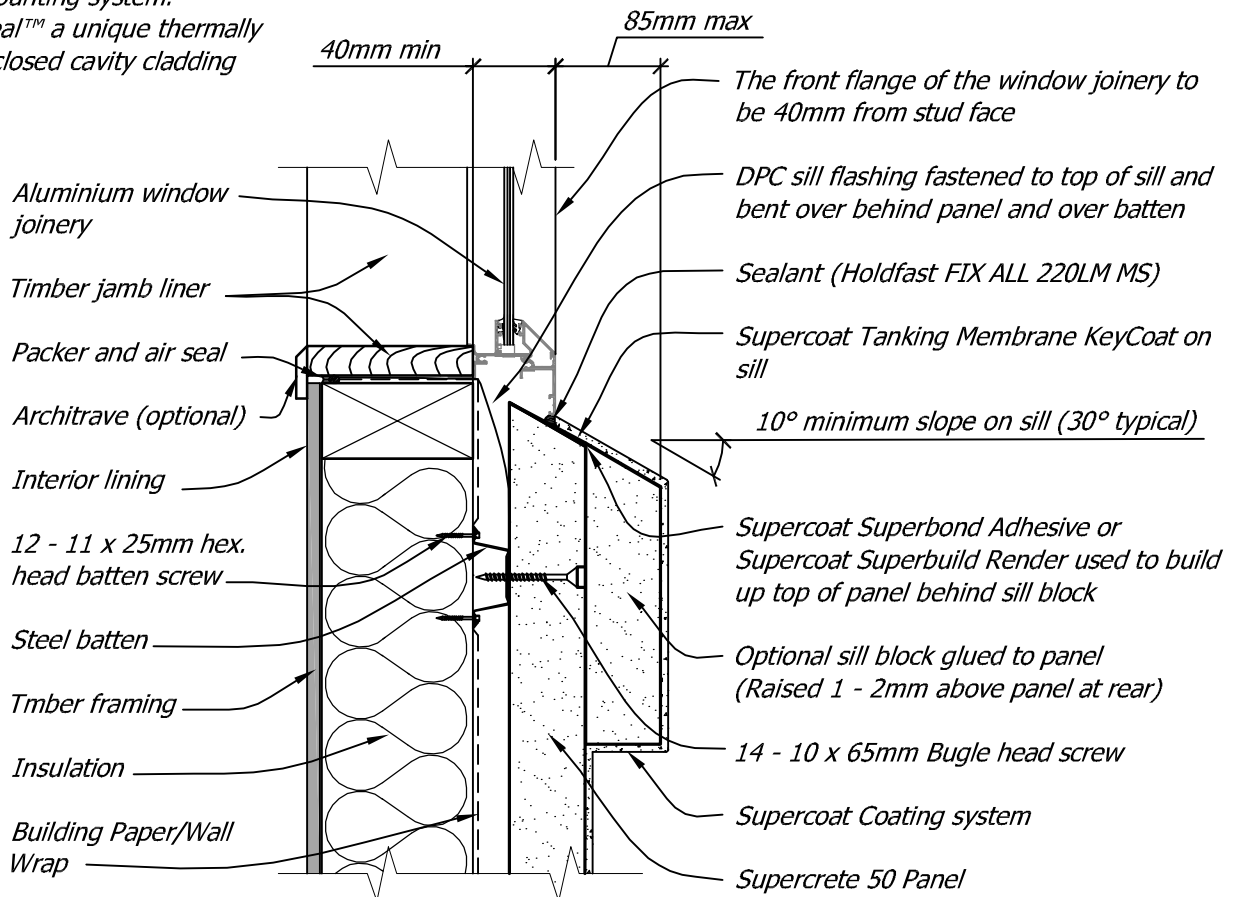
Window Sill Section
