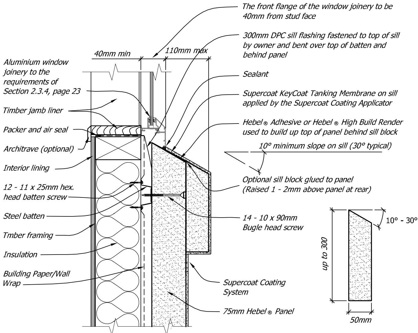
Window Sill Section
